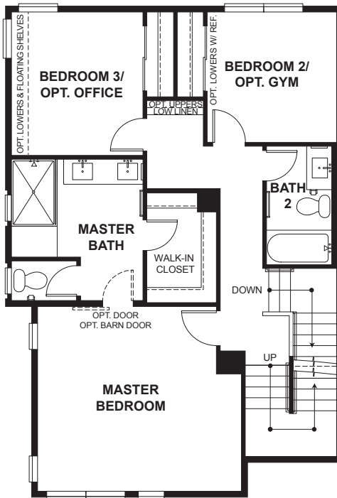
THIRD FLOOR
